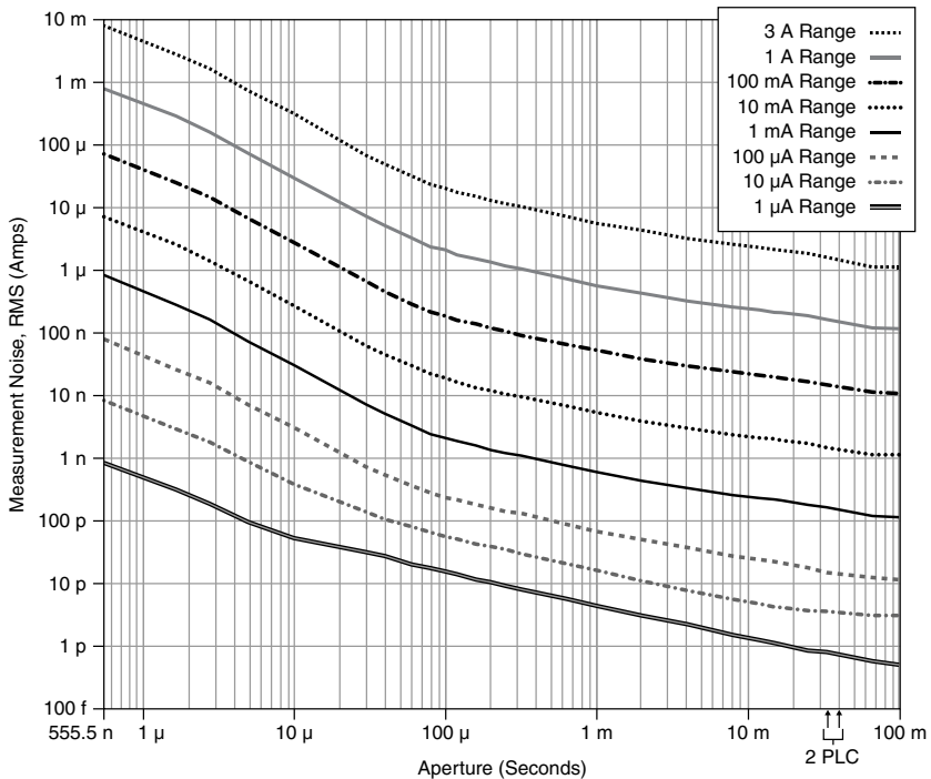
Figure 3. Current Measurement Noise vs. Measurement Aperture, Nominal
