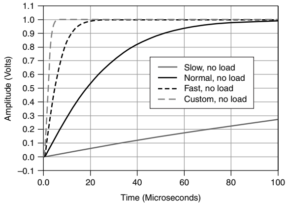
Figure 5. 1 mA Range, No Load Step Response, Nominal
